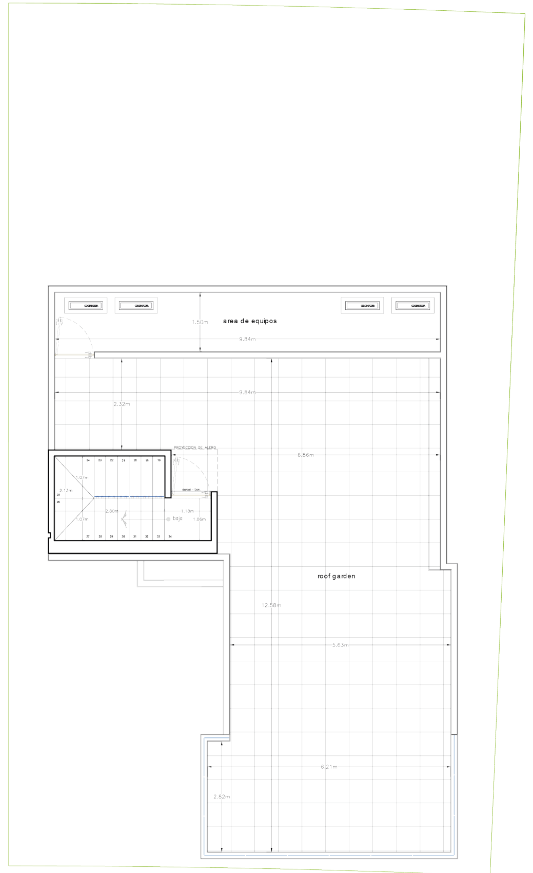
PLANTA ROOF GARDEN
